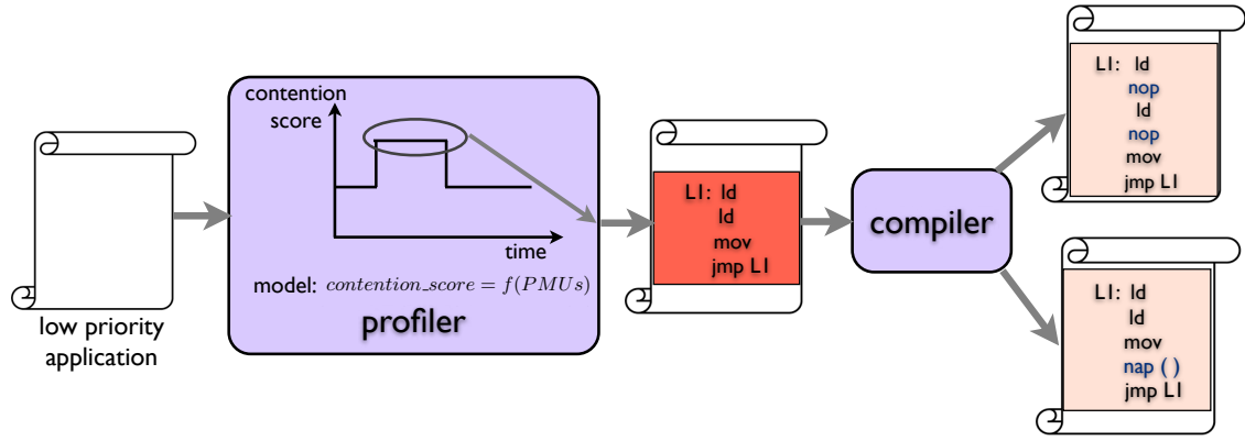
Figure 2: QoS-Compile Overview
