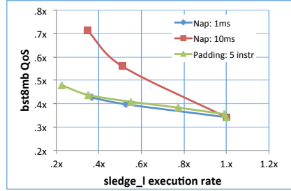
Figure 13: sledge_l padding vs. nap for bst8mb
