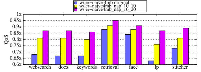
Figure 20: Google benchmark's performance when it is co-located with the original er-naive4mb, er-naive4mb with nap insertion (10ms, 10ms) and nap insertion (10ms, 20ms), normalized by each benchmark's performance when it is running alone
