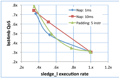
Figure 12: sledge_l padding vs. nap for bst4mb
